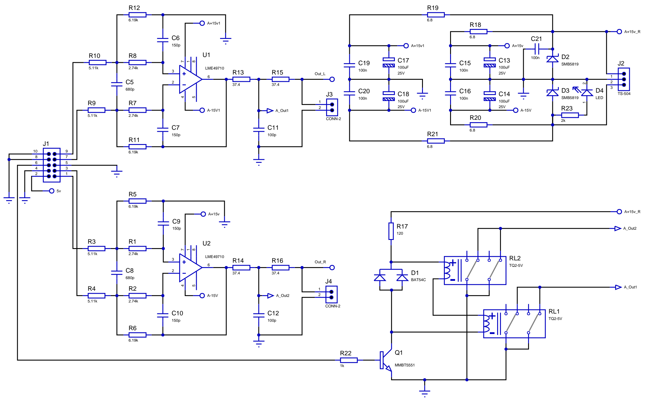
JLsounds LME49710 filter board Rev 1.0 2015
